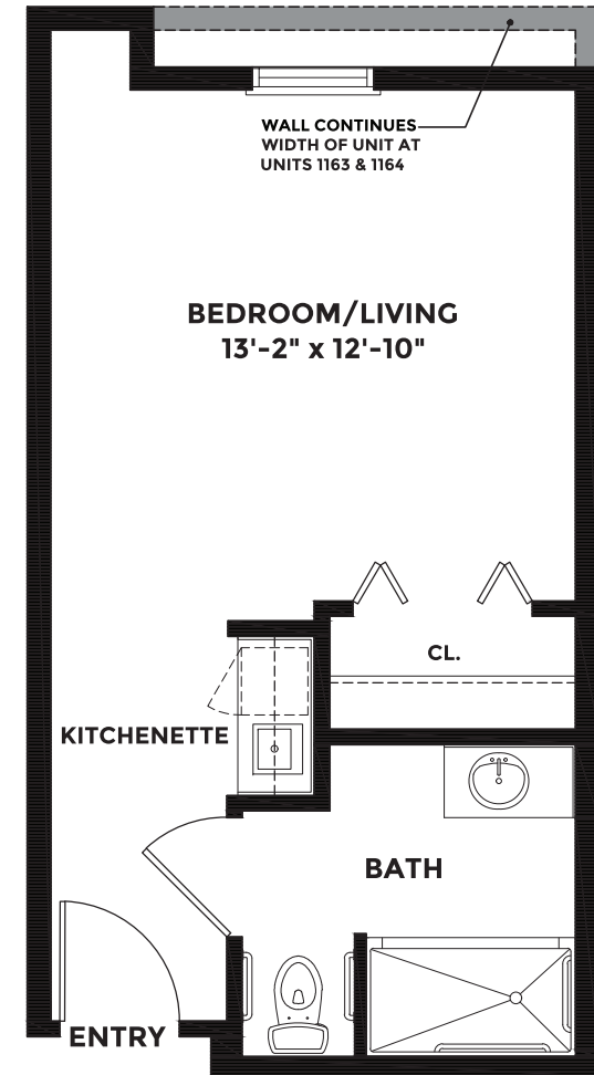
'F2' - TYPICAL PLAN
