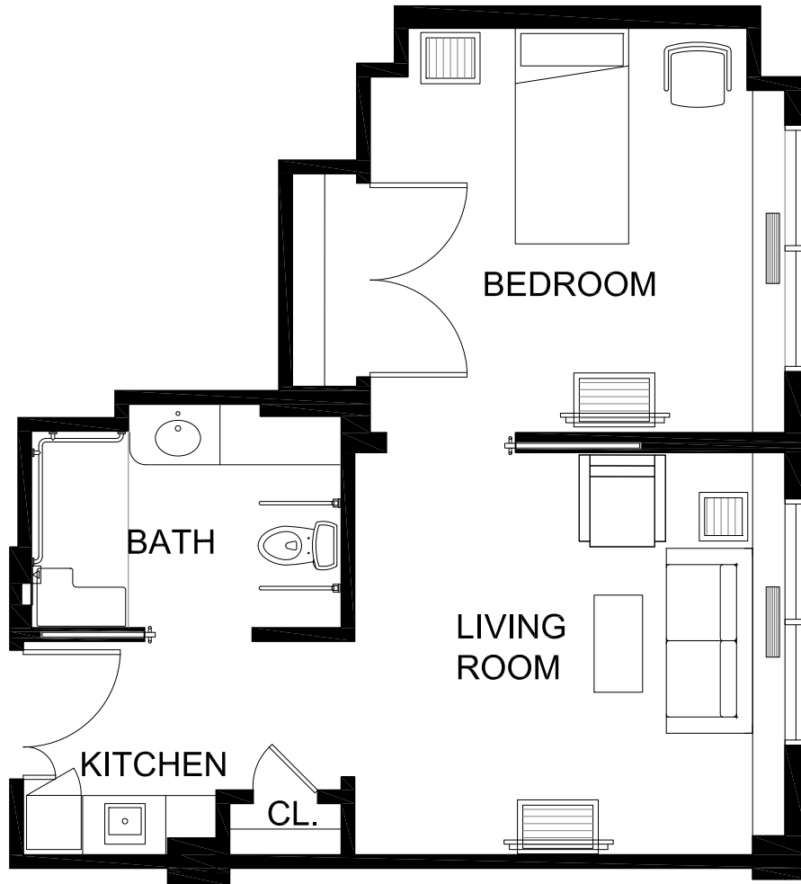
SHORT TERM CARE RESIDENT SUITE - ONE BEDROOM 487 SQFT.
