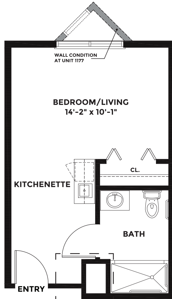
'A1' - TYPICAL PLAN
