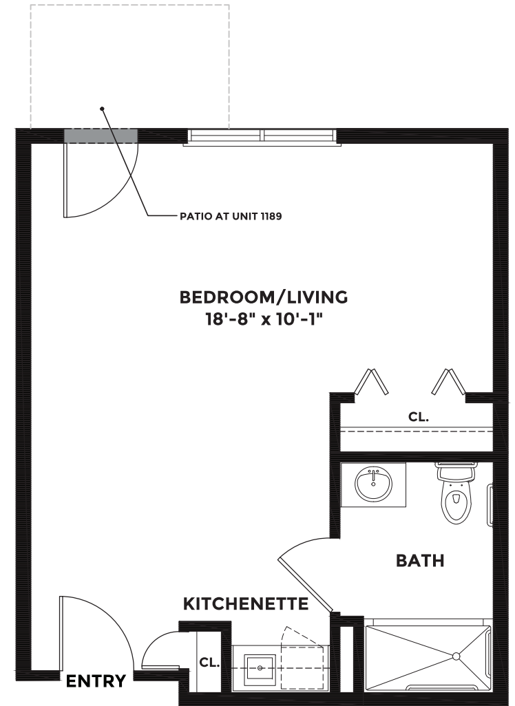
'A2' - TYPICAL PLAN
